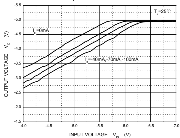
Dropout Characteristics
